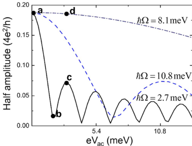
FIG. 2. (Color online) Half amplitude of the FP conductance oscillations as a function of the ac field intensity. These results are for a (24,0) metallic zig-zag nanotube of length L=440 nm and \gamma_i=0.7\gamma_0 , at zero bias voltage and temperature.
