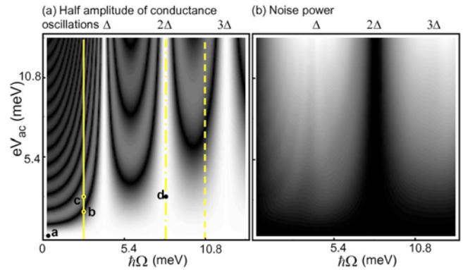
FIG. 3. (Color online) (a) Contour plot showing the half amplitude of the FP oscillations as a function of V_{ac} and \Omega at zero temperature and bias voltage. (b) Same contour plot for the current noise \bar{S} . White in both figures is for maximum values of the half amplitude and noise, respectively.
