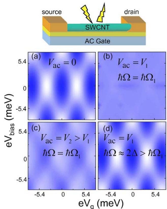
FIG. 1. (Color online) Top, scheme of the device considered in the text, a CNT connected to two electrodes and an ac gate. The panels marked with (a), (b), (c) and (d) are the FP conductance interference patterns (as a function of bias and gate voltages). The pattern observed with no ac gating [panel (a)] is modified when different driving frequencies and amplitudes are applied: (b) suppression, (c) revival and phase inversion, and (d) robustness. White and dark blue correspond to maximum and minimum conductances, respectively.
